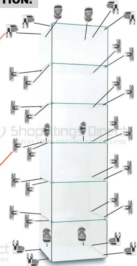
12 x Side Glass (400 x 265)
